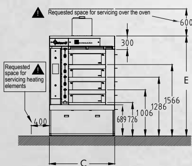
FRONT VIEW WITHOUT INTEGRATED LIFTER
