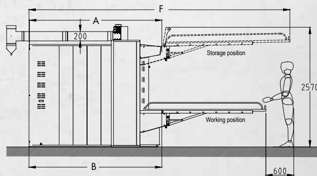
SIDE VIEW WITH INTEGRATED LIFTER
