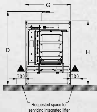
FRONT VIEW WITH INTEGRATED LIFTER
